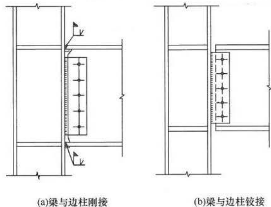
(a)梁与边柱刚接
