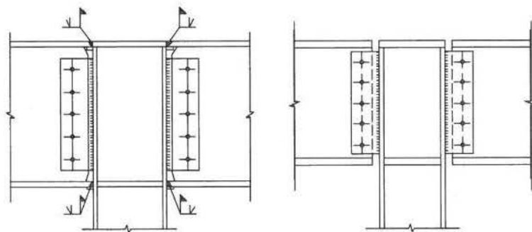
(c)梁与中柱刚接
